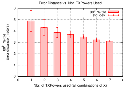
Fig. 7. The effect of varying the number of transmission power levels used to transmit beacons. Increasing the diversity of beacon power levels increases accuracy considerably.
